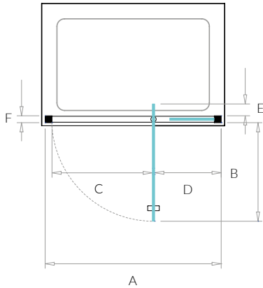
Pivot Wide Door Diagram
